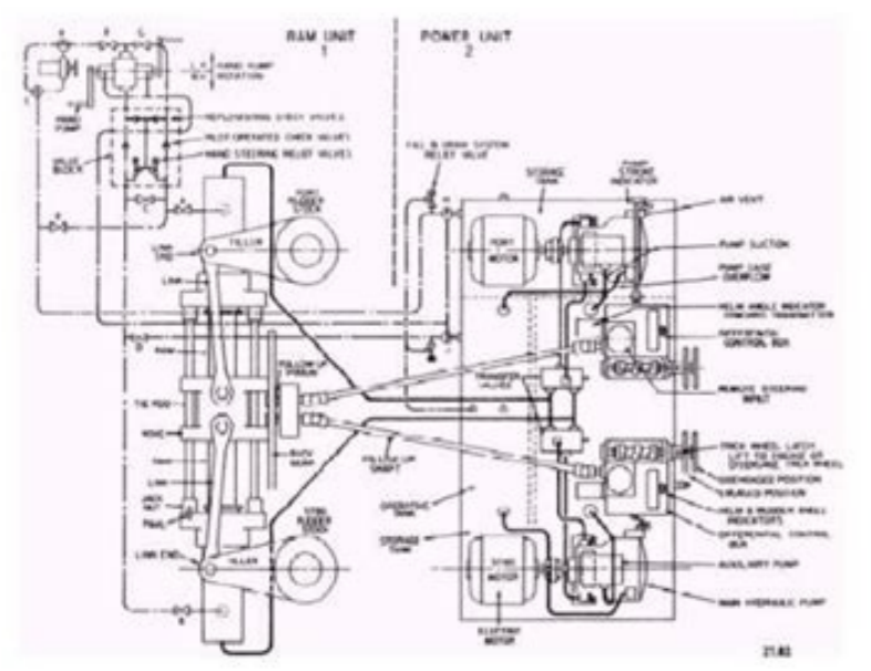
Figure 18-2. Electrohydraulic steering engine. consists essentially of (1) a ram unit and (2) a power unit. Ram Unit
